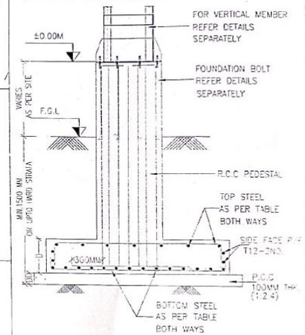
TYPICAL DETAIL OF COLUMN SECTION
